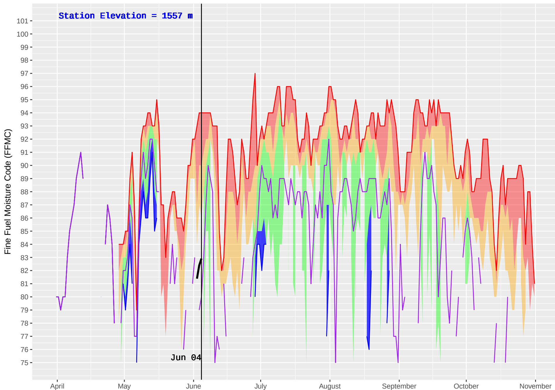
SKOONKA (1024) : Historical (2008–2016) and Current (2018) Noon Fine Fuel Moisture Code (FFMC)
